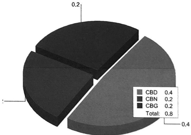
Cannabinoids Profile
